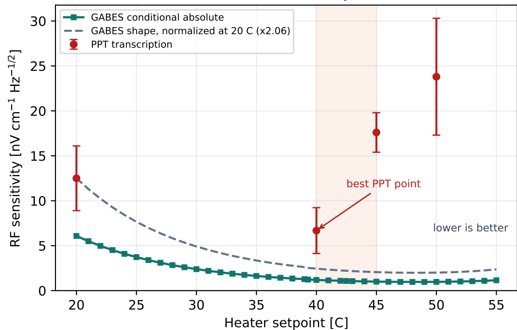
(b) RF sensitivity
