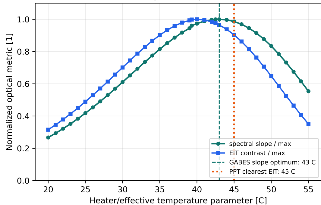
(a) Optical response
